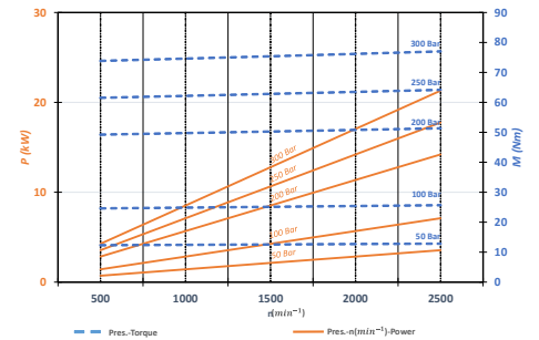
Power-Pressure Graphic
