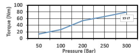
Torque-Pressure Graphic
